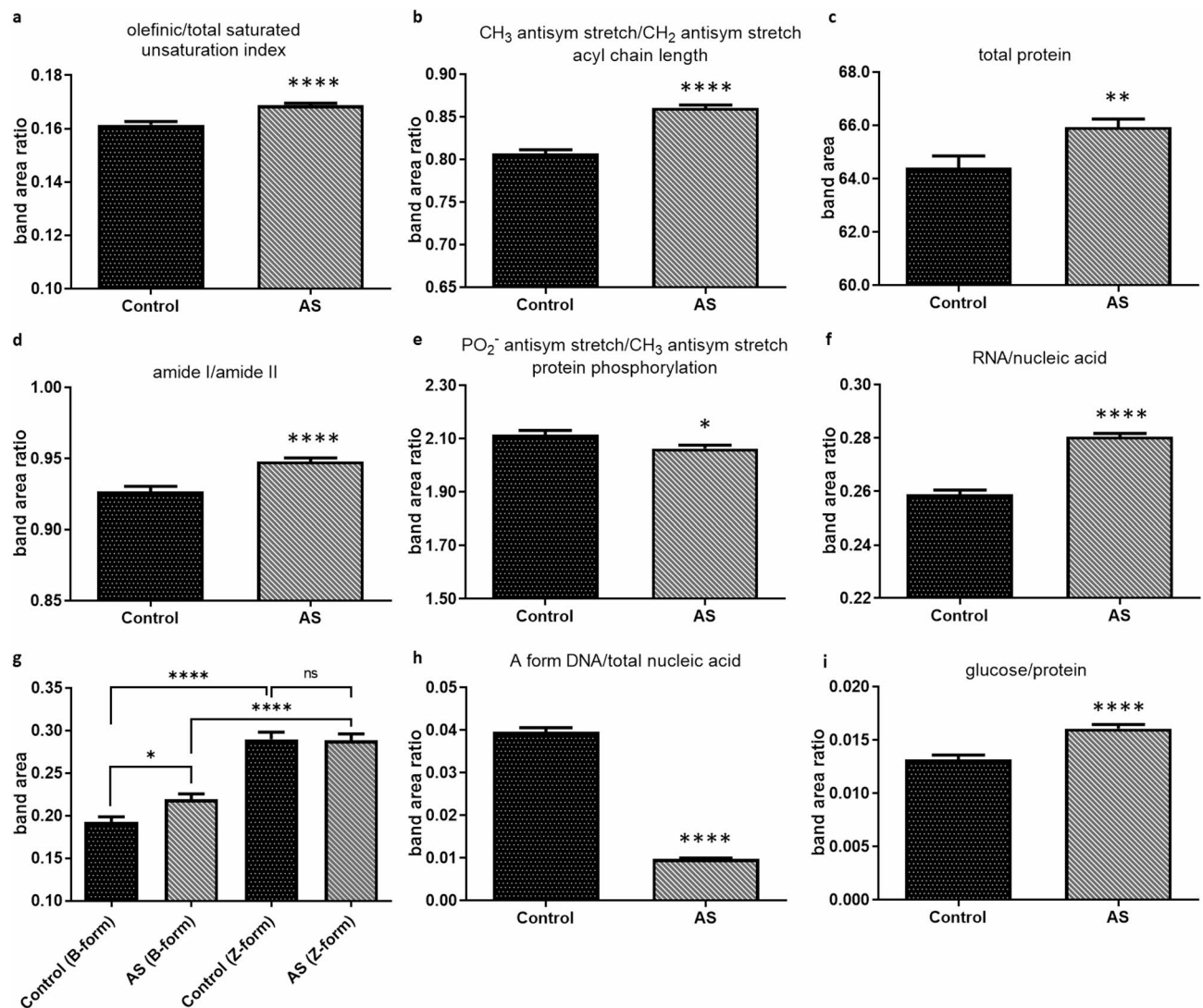
Fig. 2. Lipid, protein, and nucleic acid alterations in as vs. control groups. Bar graphs showing: (a) olefinic/total saturated lipid area ratio, (b) methyl/methylene area ratio, (c) total protein area, (d) amide I/ amide II area ratio, (e) PO 2 - antisymmetric stretching/CH 3 antisymmetric stretching area ratio, (f) RNA/nucleic acid area ratio, (g) comparison of the bands areas B-form and Z-form DNA, (h) A-form DNA/nucleic acid ratio, and (i) glucose/protein area ratio of control and AS groups (The degree of significance for the comparison of the AS group with respect to the control group was denoted as * p < 0.05 , ** p < 0.01 , *** p < 0.001 , **** p < 0.0001 ).
