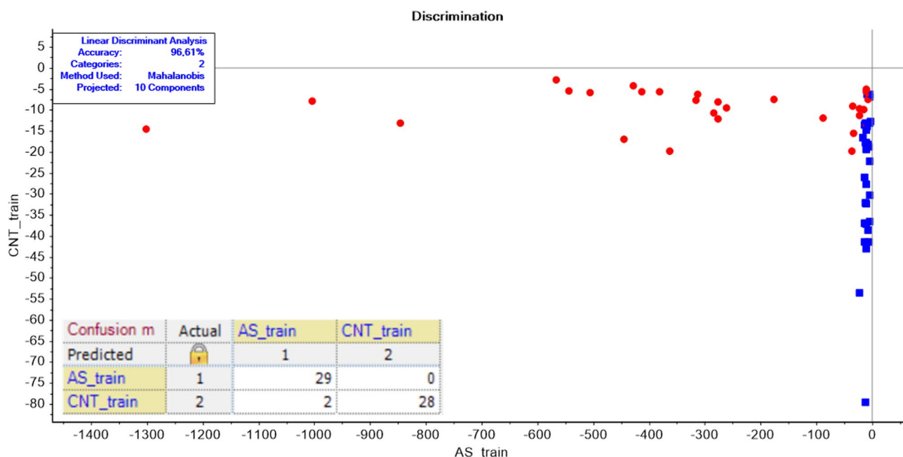
Fig. 4. Discrimination plot and confusion matrix for serum samples from the AS and control group in the 1300–800 \text{cm}^{-1} region are shown. Control (CNT) and atherosclerosis (AS) are compared.
