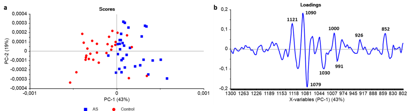
Fig. 3. PCA (a) scores and (b) loading plots for FTIR spectra of control and AS groups in the 1300\text{--}800\text{ cm}^{-1} spectral region.
