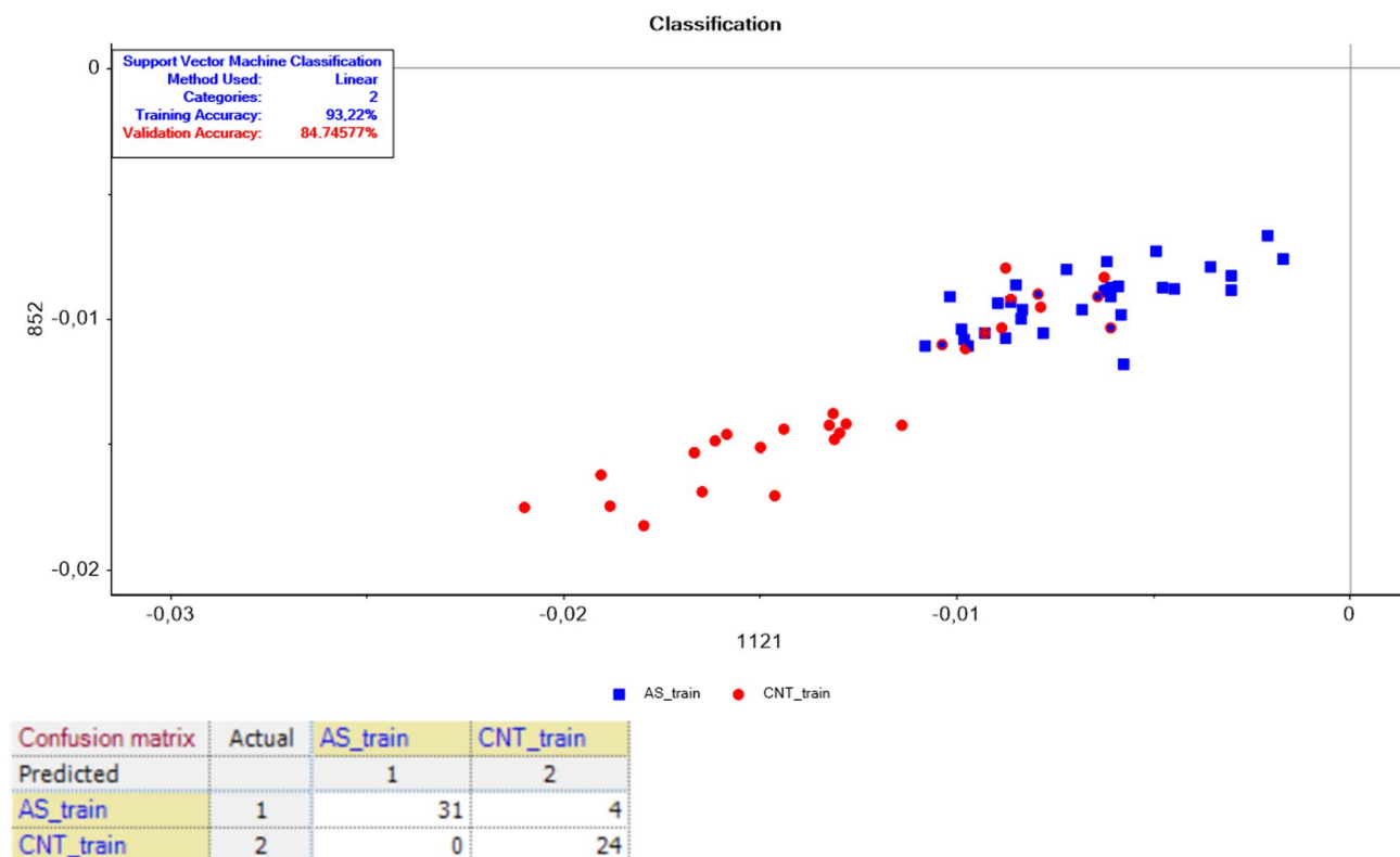
Fig. 5. SVM classification plot and confusion matrix for serum samples from the AS and CNT group in the 1800–800 \text{cm}^{-1} region.
