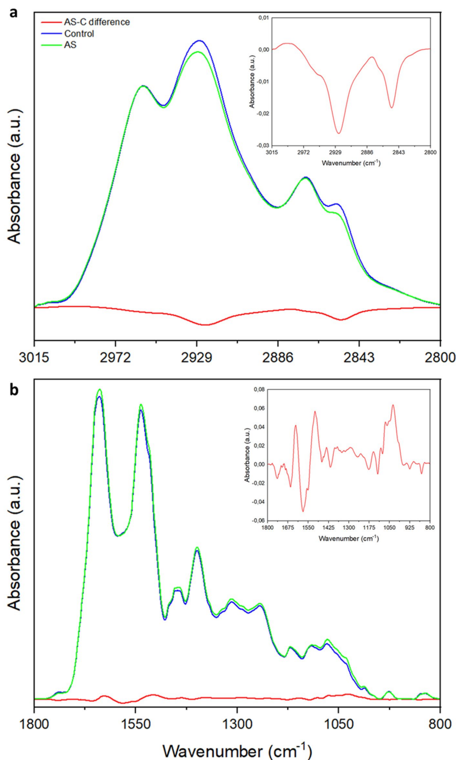
Fig. 1. Average serum spectra of the control and AS groups in (a) the 3015–2800 and (b) the 1800–800 \text{cm}^{-1} regions. The spectra were normalized to the amide A band located at 3286 \text{cm}^{-1} . Difference IR spectra for both regions, shown in the subpanels, were obtained by the subtraction of the control spectrum from AS patients' spectra. Control (blue), AS (green) and difference (red) spectra are displayed.
